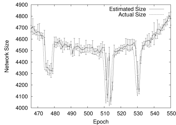
Fig. 13. Network size estimation with protocol COUNT in the presence of churn according to a Gnutella trace [Saroiu et al. 2003]. 50 experiments were run to calculate statistics (mean, and standard deviation), each epoch consisted of 30 cycles; each cycle lasted for 10 seconds.
