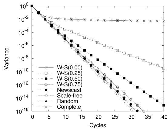
Fig. 8. Variance reduction for a network of 10^5 nodes. Results are normalized so that the initial variance is one in each experiment. Each curve corresponds to a different topology where W-S(\beta) stands for the Watts-Strogatz model with parameter \beta .
